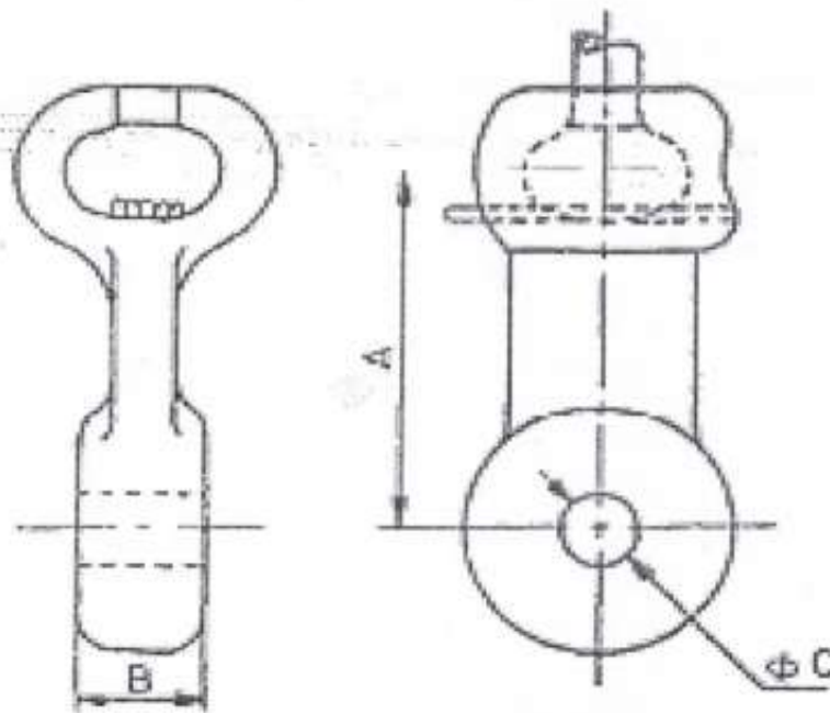
Fig-3: Socket Tongue
