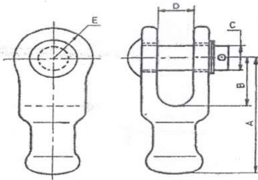
Fig 2: Ball Clevis
